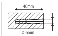
Mounting to wall / Wandmontage
