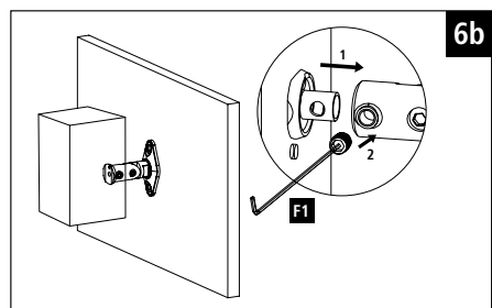
Wall mounting Wandmontage
