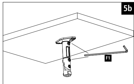
Distance 140mm Abstand 140mm
