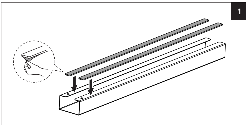
Mounting by magnetic stripes / Montage per magnetische Streifen
